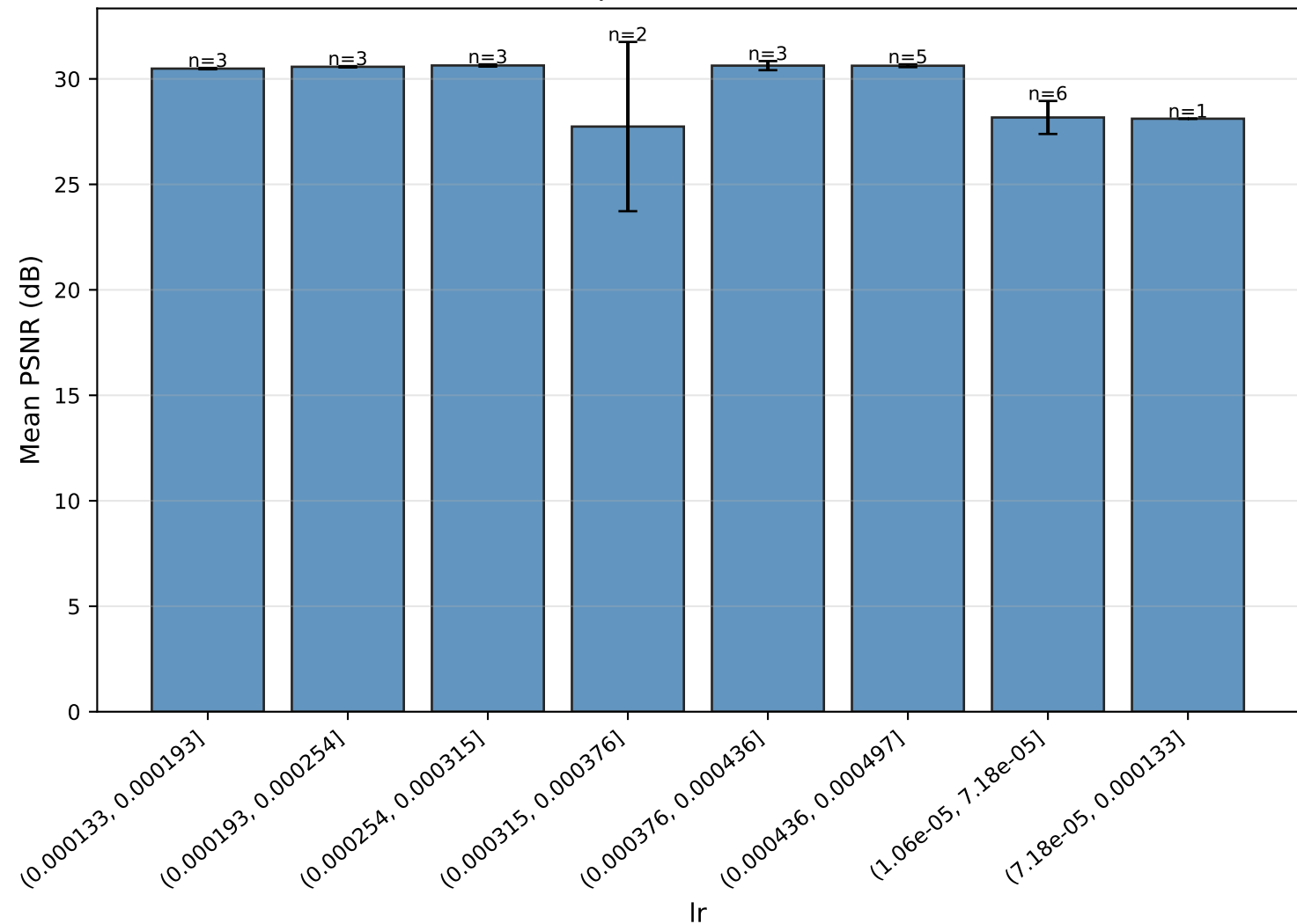
Mean PSNR per value of l_r — OmniSR
